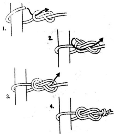
Figure 8 follow through
